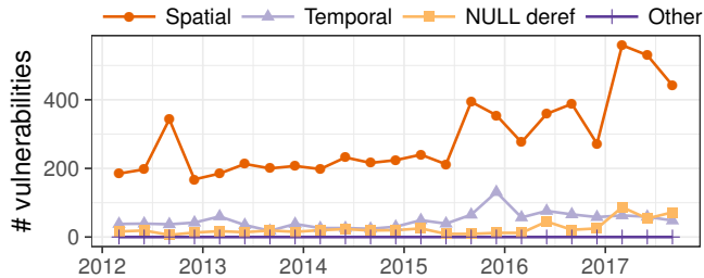
Figure 1. Number of reported vulnerabilities in the CVE database (2012-03 to 2017-09).
